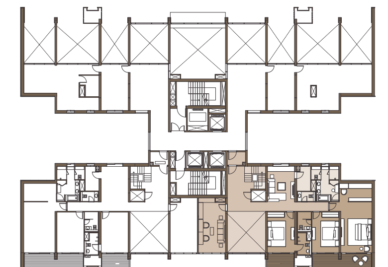
5 BEDROOM PODIUM VILLA APARTMENT LEVEL 2 FLOOR LAYOUT
